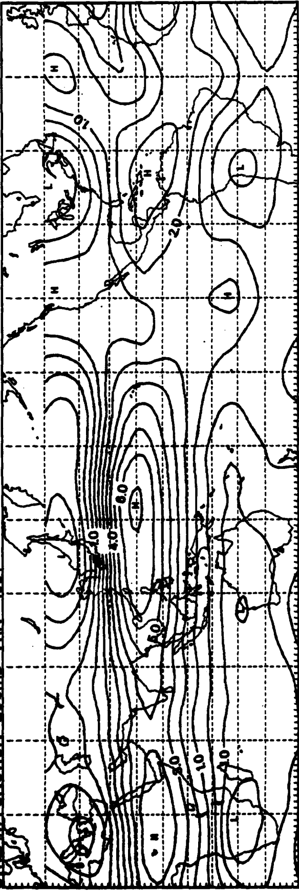
STREAM FUNCTION 200MB WIN 1981
